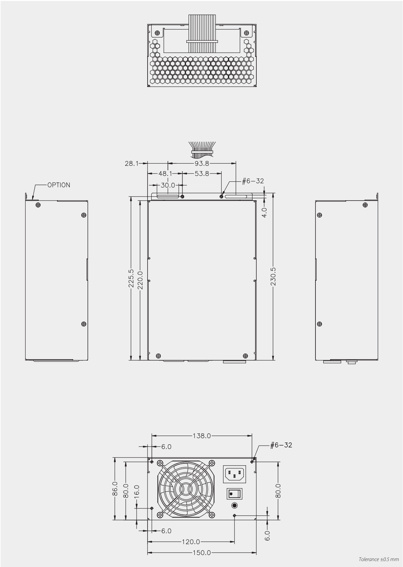
Drawing PSL-6A00V
